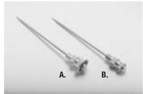
Linkert Low Speed Needle Valve Accurate reproduction of OEM 27340-33 needle valve used on all 1933-1947 1" carburetors. 3-1/16" long needle available with Type 1 or Type 2 head. A. Stock No. 2707-5 Type 1 B. Stock No. 2708-5 Type 2
